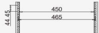
Mounting Dimension
