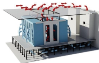
Hot aisle containment
