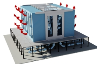
Cold aisle Containment
