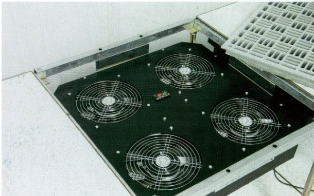
4 Four-Fan Unit
